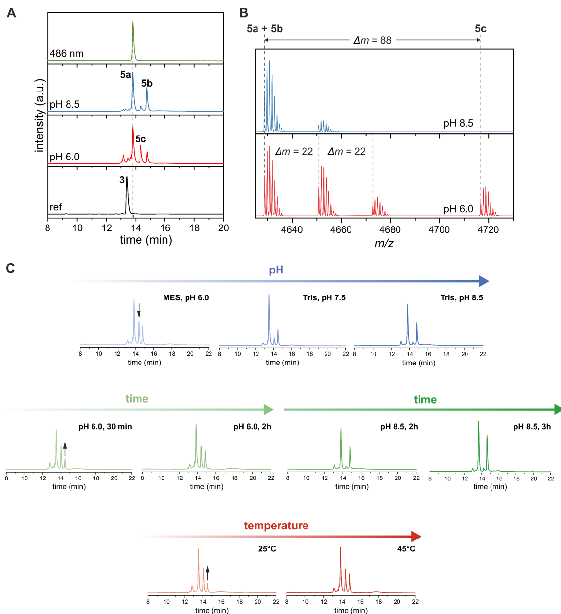
Figure S5. Optimization of the synthesis of chromophore 5 on RNA. A Anion-exchange HPLC analysis of the generation of chromophore 5a in Ne-RNA R1 with formation of side products 5b and 5c conducted at pH 6.0 (red trace, monitored at 260 nm) or at pH 8.5 (blue trace, monitored at 260 nm, and green trace at 486 nm ( \epsilon_{486\text{ nm}} \sim 6 \times 10^4 \text{ L} \cdot \text{mol}^{-1} \cdot \text{cm}^{-1} )). Unmodified reference R1 monitored at 260 nm shown in black. B Deconvoluted HR-ESI-MS spectra of the isolated products for the Ne-RNA R1 reaction that was conducted at pH 8.5 (top, blue trace) or pH 6.0 (bottom, red trace). \Delta m = 22 denotes Na + -adducts. C Anion-exchange HPLC analysis of PAGE-purified modification products. Ne-RNA R1 was first reacted overnight with MTR1 in the presence of Br 6 G followed by reaction with 4 under different conditions, as indicated by variation of pH, reaction time or temperature. The standard set of conditions were (unless otherwise mentioned): 85 \mu\text{M} substrate RNA in 25 mM MES (pH 6.0), 100 mM KCl and 75 mM 4 at 45 °C for 2h.
