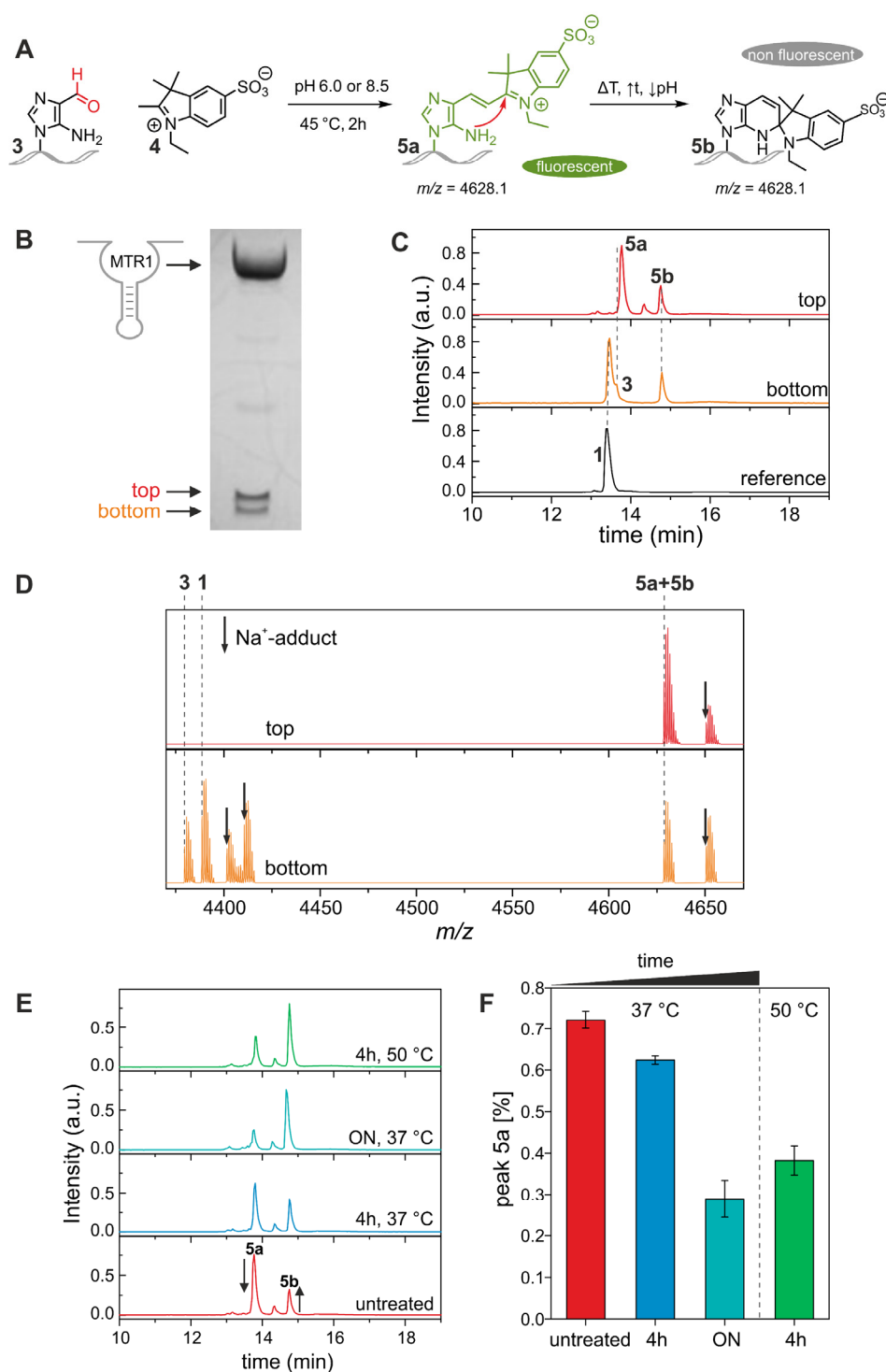
Figure S6. Conversion of chromophore 5a to the isomeric spiro compound 5b. A Proposed reaction mechanism for the generation of the isomeric non-fluorescent spiro compound 5b that is favored under elevated temperatures ( \Delta T ), longer reaction times ( \uparrow t ), and lower pH ( \downarrow \text{pH} ). B Purification of MTR1 + Bn 6 G treated Ne-RNA R1 reacted with 4 on denaturing PAGE. C Anion-exchange HPLC analysis of RNA fractions isolated from B (all traced monitored at 260 nm). D Deconvoluted HR-ESI-MS spectrum of RNA fractions isolated from B . Arrows denote sodium adducts. E Monitoring the conversion of 5a to 5b in the “top” RNA fraction from B using anion-exchange HPLC (260 nm). The RNA was incubated at pH 8 under elevated temperatures followed by analysis with anion-exchange HPLC. F Analysis of the peak areas corresponding to 5a and 5b from E .
