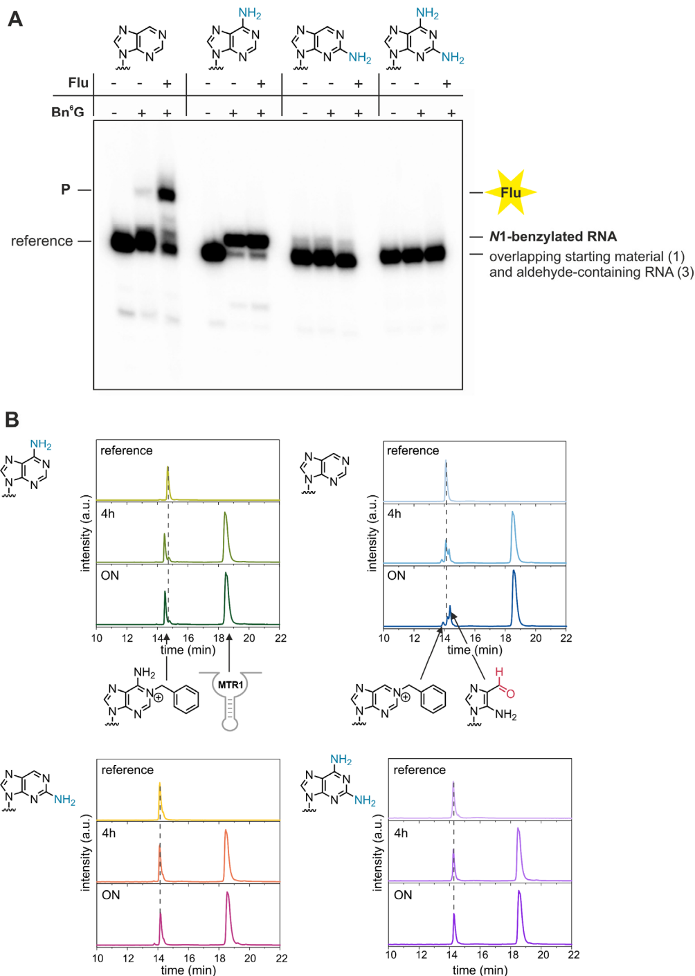
Figure S1. Reactivity of atomic nebularine mutants. A. Atomic mutagenesis of the RNA R2. The 5'-32P-labeled RNAs containing either A, Ne, 2AP or DAP at the target site were incubated with MTR1 at 25 °C for 23 h in the presence (+) or absence (-) of Bn 6 G followed by labelling with Flu-TSC (+). P = fluorescently labelled reaction product B. Anion-exchange HPLC analysis of MTR1-catalyzed reaction of RNA R2 atomic mutants with A, Ne, 2AP or DAP as target sites. N1-benzylated RNA elutes earlier than reference (for A (upper left dataset). Aldehyde-containing RNA elutes later than reference (for Ne, upper right dataset). 2AP and DAP do not show any conversion in PAGE and HPLC analyses.
