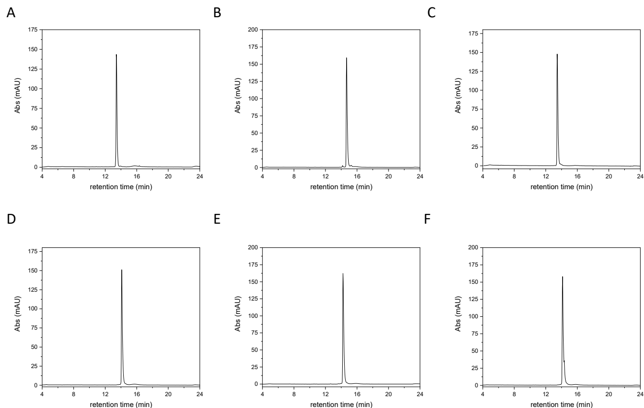
Anion exchange HPLC chromatograms to confirm purity of RNA oligonucleotides prepared by solid-phase synthesis. (A) R1_un, (B) R2_un, (C) R1_Ne, (D) R2_Ne, (E) R2_DAP, (F) R2_2AP. Dionex DNAPAc PA200, 2x250 mm, 60°C, monitored at 260 nm.
