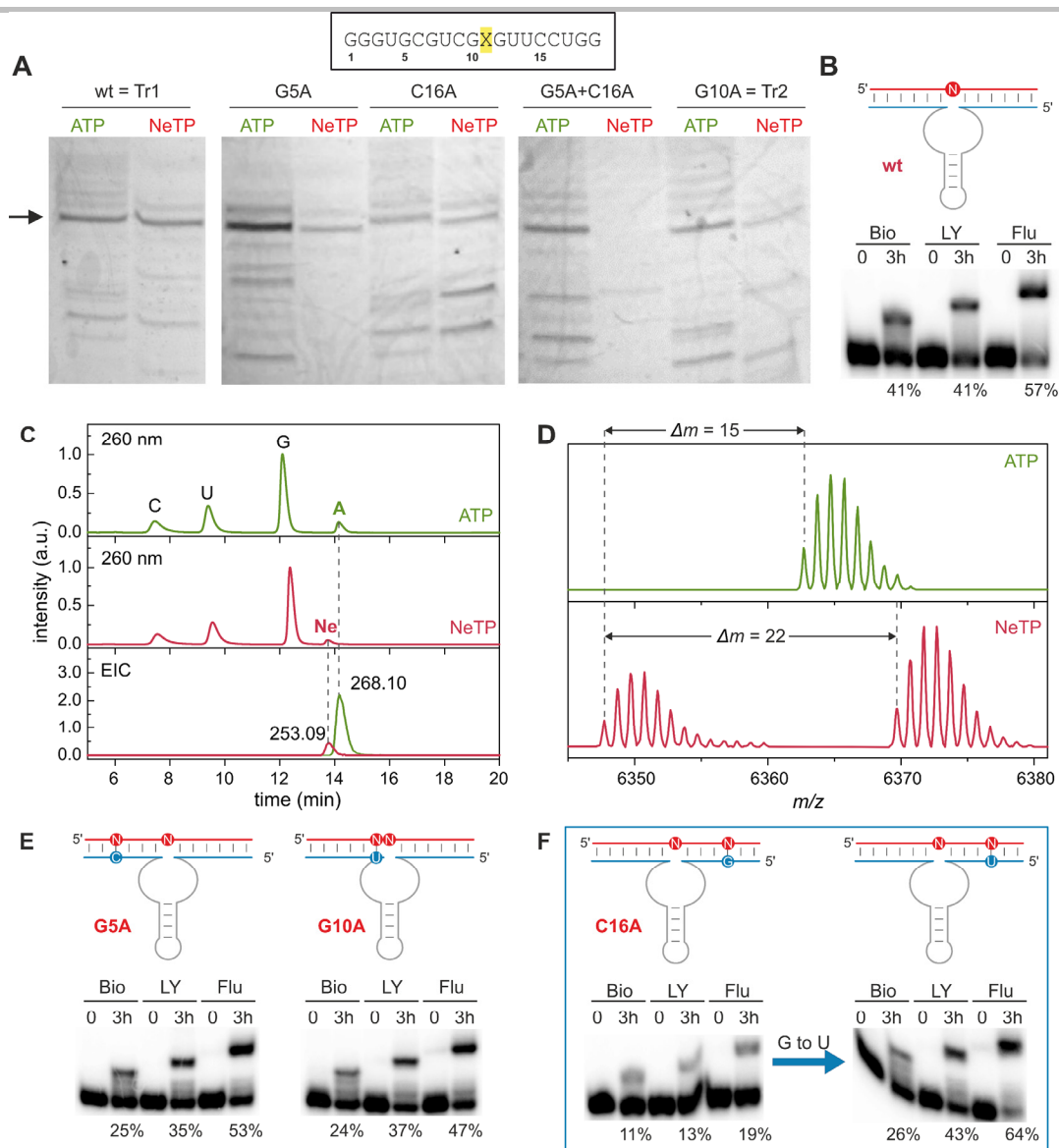
Figure S7. In vitro transcription using NeTP and modification of the transcripts. A Purification of a 19-mer substrate RNA Tr1 and its point mutants transcribed using ATP or NeTP. X denotes incorporation site of A or Ne in the wild type (wt) RNA Tr1. Arrow indicates the desired product. B Aldehyde functionalization of MTR1 + Bn 6 G Ne-transcript Tr1 using Bio-hyd. (Bio), LY-CH (LY) or Flu-TSC (Flu). C LC-MS analysis of digested unreacted ATP and NeTP wt transcript Tr1. UV traces at 260 nm and EICs ( m/z 253.09 \pm 0.01; corresponding to Ne and m/z 268.10 \pm 0.01 corresponding to A) are shown. D Deconvoluted HR-ESI-MS spectra of wt ATP and NeTP Tr1 transcripts, containing a single adenosine or nebularine, respectively. As expected, the Ne-Tr1 is lighter by 15 mass units. \Delta m = 22 denotes Na + adduct. E Aldehyde functionalization of MTR1 + Bn 6 G treated Ne-Tr1 and its point mutants with Bio-hyd, LY-CH or Flu-TSC. Circles denote Ne incorporation sites (N; red) and the respective base-pairing partner in the ribozymes binding arm (blue). F Aldehyde functionalization of MTR1 + Bn 6 G treated Ne-Tr2 (= G10A mutant) with Bio-hyd, LY-CH or Flu-TSC. The G to U point mutation in the ribozymes binding arm restored the labelling efficiency.
