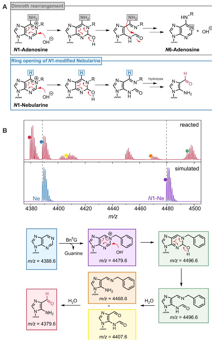
Figure S2. Mechanism of the MTR1 ribozyme-catalyzed aminoimidazole aldehyde generation. A Reaction mechanism of the Dimroth rearrangement of N 1 - to N 6 -modified adenosine. The analogous reaction of N 1 -modified nebularine results in a ring-opened intermediate, which is hydrolyzed. B Deconvoluted HR-ESI-MS spectrum of the isolated MTR1 + Bn 6 G treated Ne-RNA R1 (top) and the simulated references of respective unmodified or N 1 -benzylated Ne-RNA R1 (bottom) together with the proposed reaction mechanism derived thereof. Note: C2 is expected to be more electrophilic than C6. However, in an alternative mechanism, the first attack of H 2 O (or OH - ) could also occur at C6 instead of C2, which would lead to isomeric intermediates with same mass, and result in the same final product.
