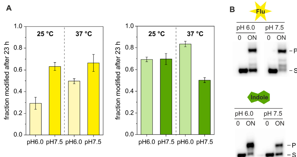
Figure S4. One-pot modification reactions. A Analysis of one-pot Ne-modification reactions in Ne-RNA R1 using Flu-TSC (yellow) or 4 (green). Reactions were conducted for 23 h at 25 °C or 37 °C using N,N -DMED (pH 6.0/pH 7.5) for Flu-TSC or MES (pH 6.0)/Tris (pH 7.5) for 4 . B Representative gel images from one-pot reactions performed at 37 °C. P, product; S, substrate. ON = over night, here 23 h.
