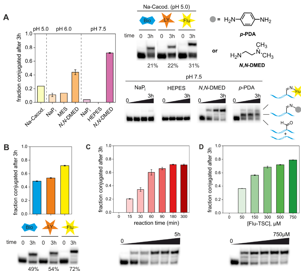
Figure S3. Optimization of the aldehyde labeling reaction. A Aldehyde functionalization using various buffers with different pH. Ne-RNA R1 was treated with MTR1 + Bn 6 G followed by reaction with Flu-TSC for 3 h at 37°C. B Aldehyde functionalization on Ne-RNA R1 treated with MTR1 + Bn 6 G using Flu-TSC in N,N -DMED (pH 7.5) for 3 h at 37°C. C Time dependency of the aldehyde functionalization in Ne-RNA R1 in N,N -DMED (pH 7.5) using 500 \mu\text{M} Flu-TSC with incubation at 37°C. D Flu-TSC concentration dependency of the aldehyde functionalization in Ne-RNA R1 in N,N -DMED (pH 7.5) with 3 h incubation at 37°C.
